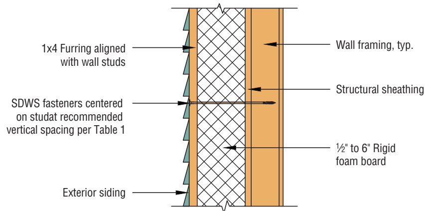
Figure 2: Furring and Rigid Foam Attachment Detail
