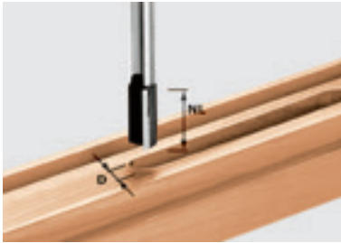
Router cutter HW with fitted base blade, shank 12 mm
