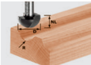
Flute cutter HW, shank 8 mm
