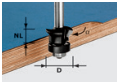
Chamfer/edge trimming cutter with ball bearing guide, shank 8 mm
