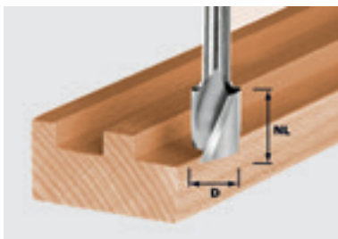
Spiral router cutter HS with base blade, shank 8 mm
