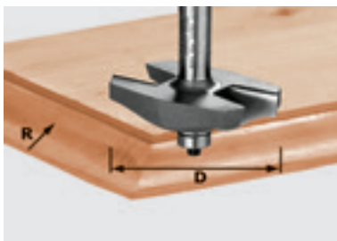
Plane cutter HW with ball bearing guide, shank 12 mm HW s = 12
