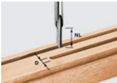
Router cutter HS single-edged, with base blade, shank 8 mm
