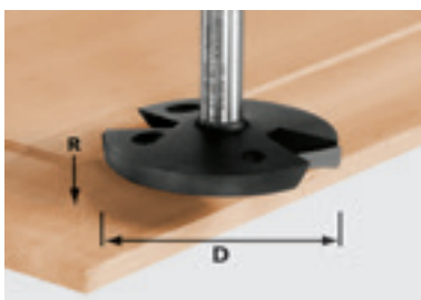
Facing cutter HW, shank 12 mm HW s = 12
