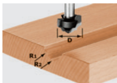
Profile cutter HW, shank 8 mm
