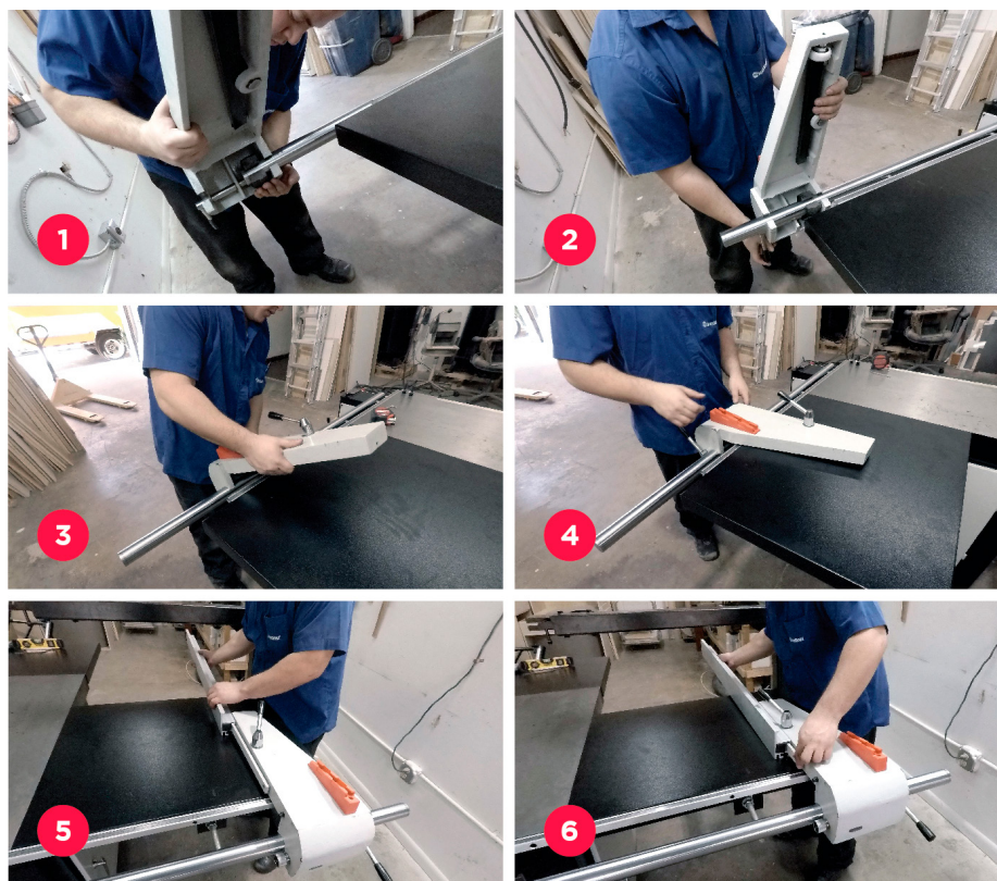
Fig. 1, 2, 3 and 4: Position the guide on the support table.
