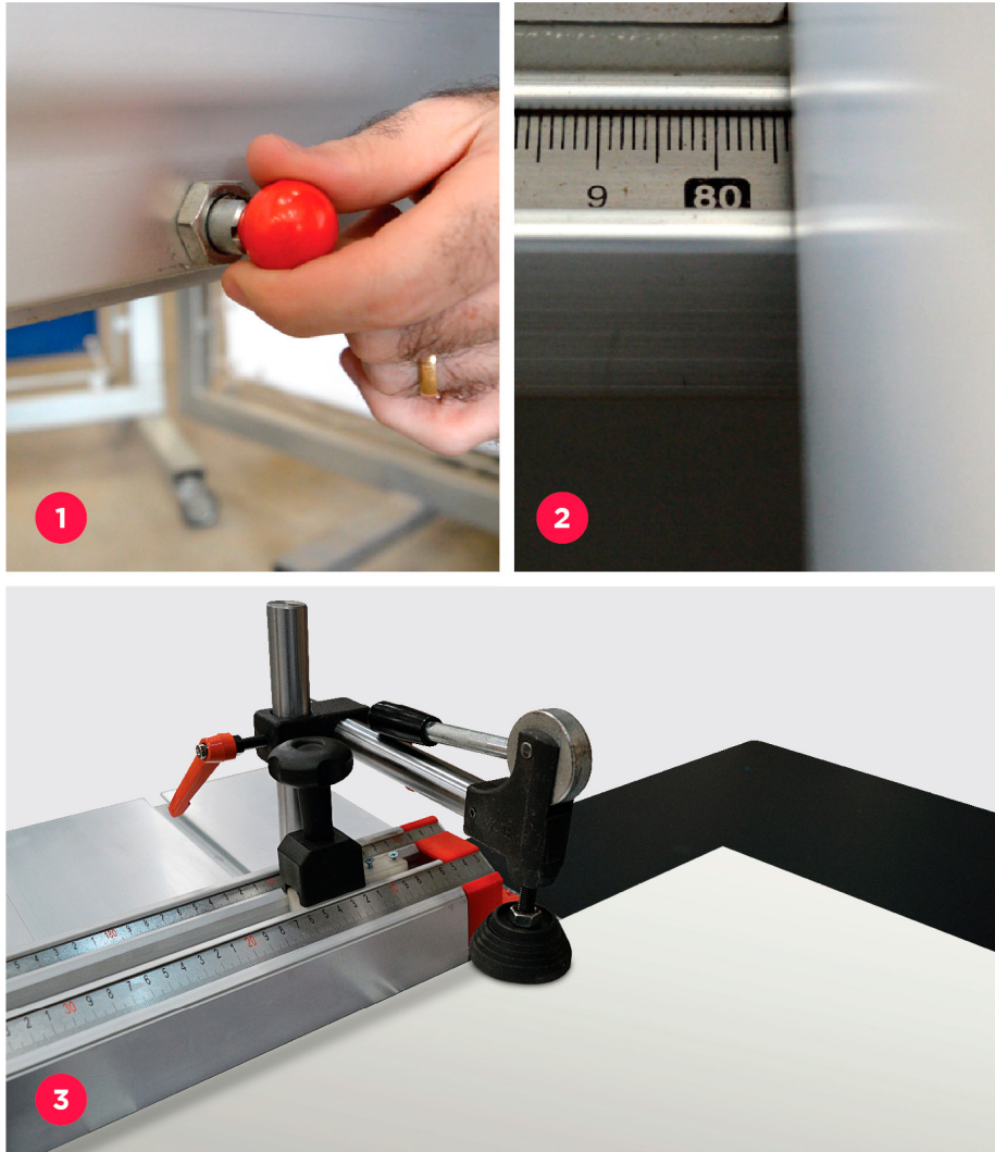
Fig. 1: Workpiece against the fixed table guide.
