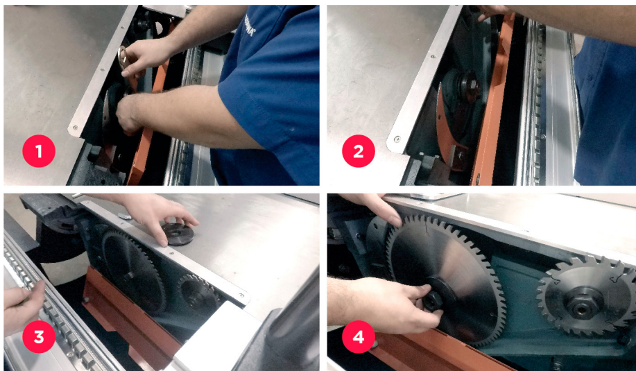
Fig. 1 and 2: Remove the nut.
