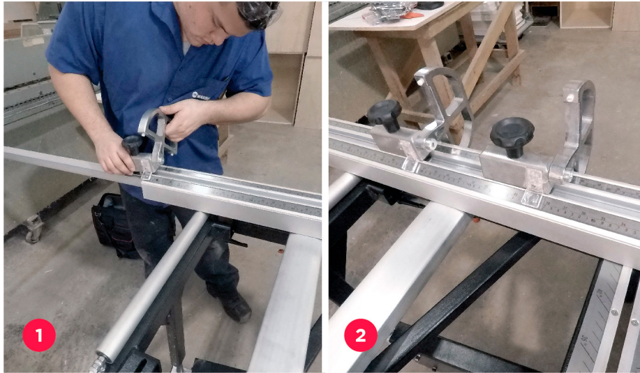
Fig. 1 and 2: Fit the wood panel stopper on the aluminum tab and tighten the handles.
