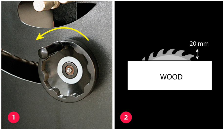
Fig. 1: Saw blade raise handle.
