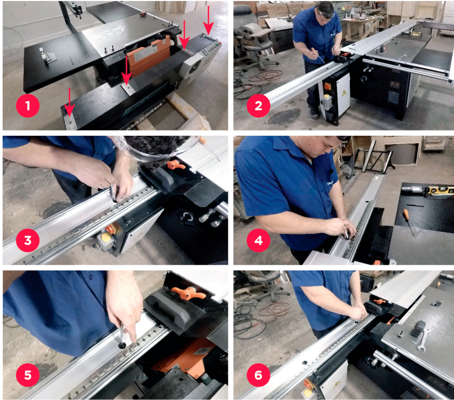
Fig. 1: Place the movable table on top of the fixed table structure, always aligning the holes with the screws.
