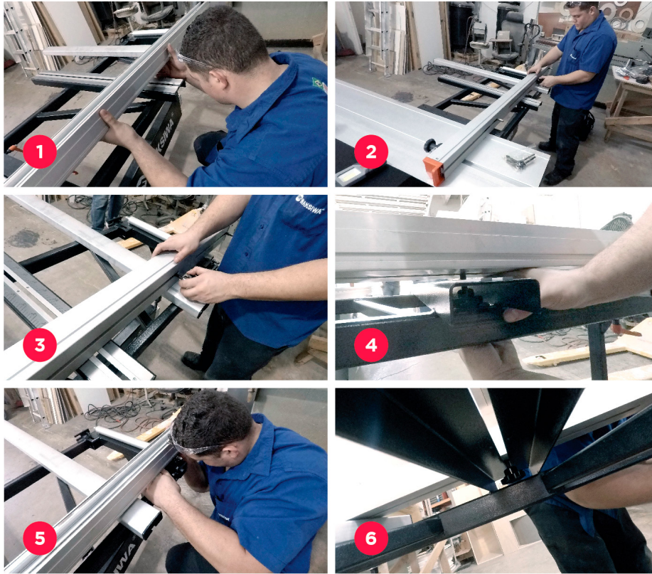
Fig. 1 and 2: Attach the aluminum tab to the movable table guide.
